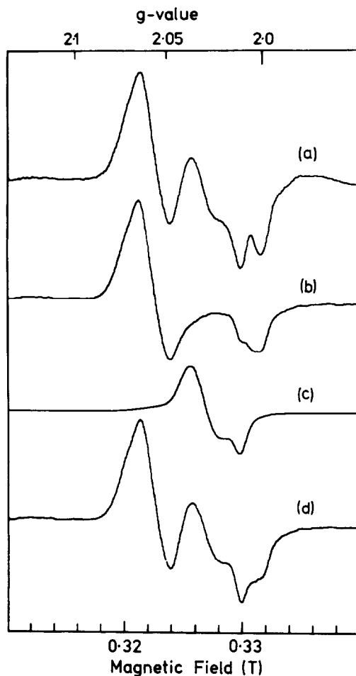
Fig.2. EPR spectra of nitrosyl-sirohaem reductase: (a) enzyme (2 mg/ml) plus 1 mM ascorbate, flushed with NO for 10 min at 20^\circ\text{C} ; (b) enzyme (2 mg/ml) plus 30 mM nitrite and 1 mM ascorbate; (c) 50 mM cysteine, 5 mM ascorbate, 25 mM nitrite and 12.5 mM ferrous sulphate, incubated at 20^\circ\text{C} for 10 min; (d) computed addition of (b) and (c). Conditions of measurement, as in fig.1, except modulation amplitude at 1.0 mT, so that the nitrogen hyperfine splitting is not visible.
