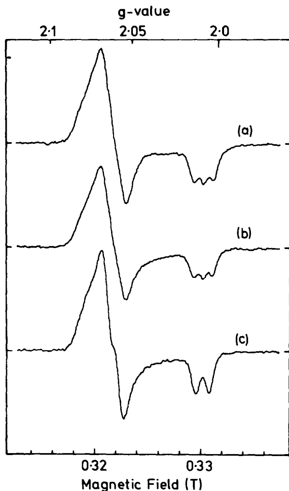
Fig.3. Exchange of ^{14}\text{NO} in the ^{14}\text{NO} -sirohaem complex with \text{Na}^{15}\text{NO}_2 . A sample of enzyme (2 mg/ml) was treated with 30 mM \text{Na}^{14}\text{NO}_2 and 3 mM \text{Na}_2\text{S}_2\text{O}_4 at 20^\circ\text{C} for 5 min before freezing. Spectrum (a) was recorded under similar conditions to fig.1. The treated enzyme was passed through a 10 \times 1.5 cm Sephadex G-25 column and reconcentrated on an amicon concentrator B15 (Amicon Corp. Lexington, MA 02173) at 20^\circ\text{C} to \sim 2 mg/ml, spectrum (b). The sample, in the presence of 30 mM \text{Na}^{15}\text{NO}_2 , was then reduced with 3 mM \text{Na}_2\text{S}_2\text{O}_4 for 10 min at 20^\circ\text{C} before freezing, spectrum (c).
