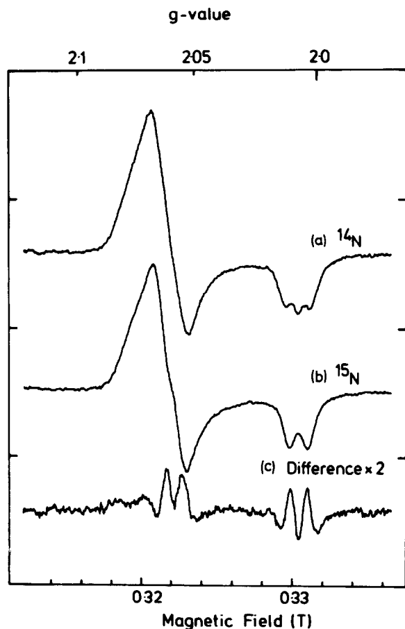
Fig.1. EPR spectra of nitrosyl-sirohaem nitrite reductase. Enzyme (3 mg/ml) treated with 30 mM \text{NaNO}_2 and 3 mM \text{Na}_2\text{S}_2\text{O}_4 at 20^\circ\text{C} for 5 min. (a) With ^{14}\text{N} nitrite; (b) with ^{15}\text{N} nitrite; (c) computed difference between (a) and (b). Conditions of measurement: temp. 30 K; microwave power 1 mW; frequency 9.28 GHz; modulation amplitude 0.16 mT; modulation frequency 100 kHz.
